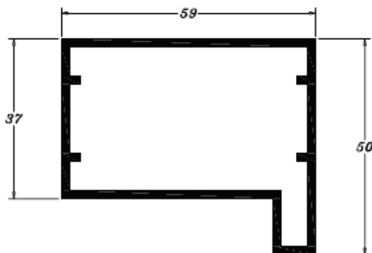
PE0861 1,192 Kg/m
